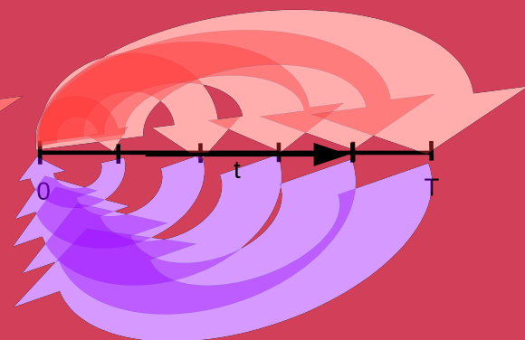
one reduced Landweber-Kaczmarz cycle
