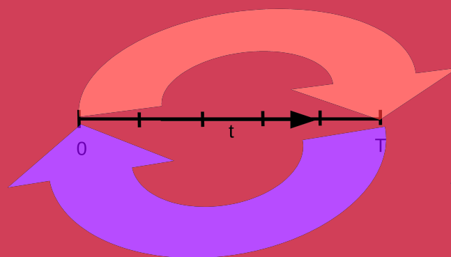
one reduced Landweber step
