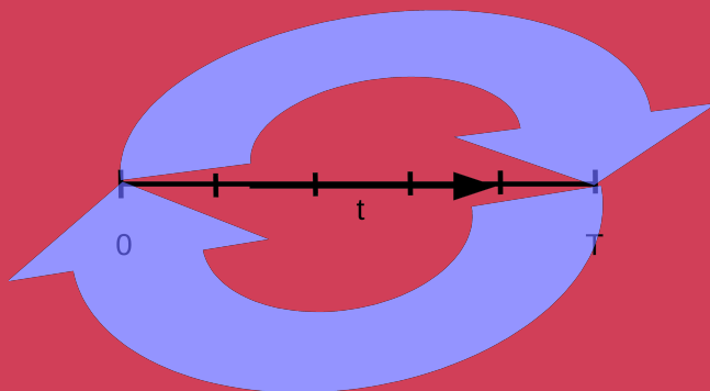
one all-at-once Landweber step
