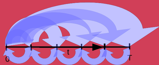
one all-at-once Landweber-Kaczmarz-cycle
